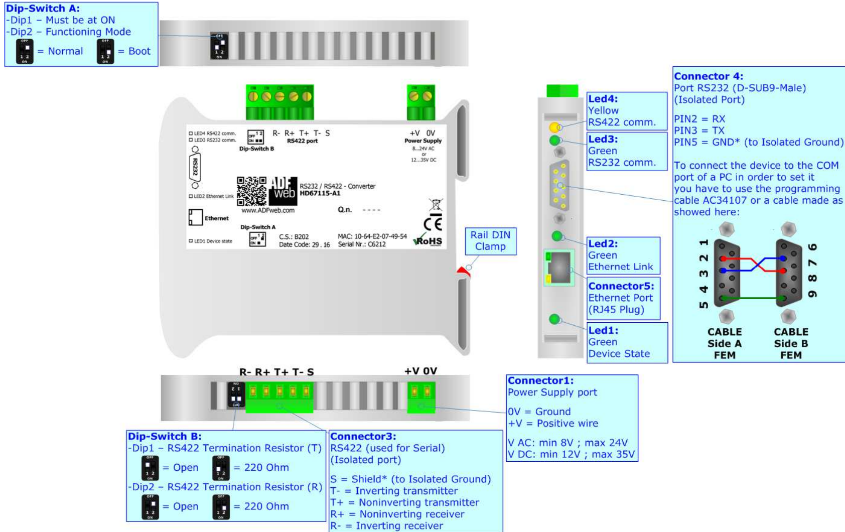
Figure 1: Connection scheme for HD67115-A1
