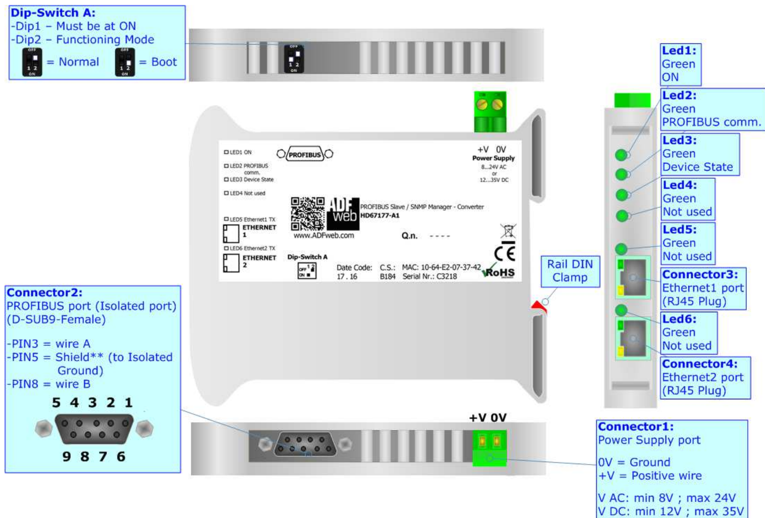
Figure 1: Connection scheme for HD67177-A1
