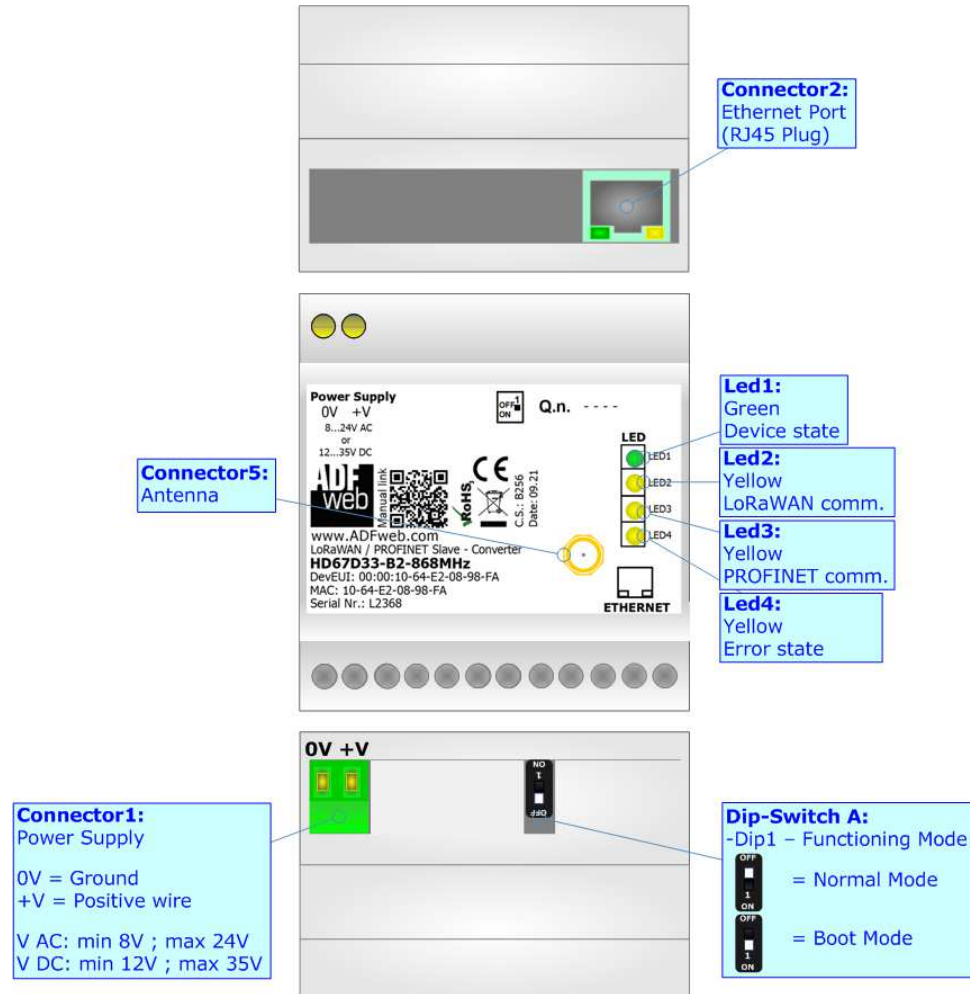
Figure 1: Connection scheme for HD67D33-B2-xxxMHz
