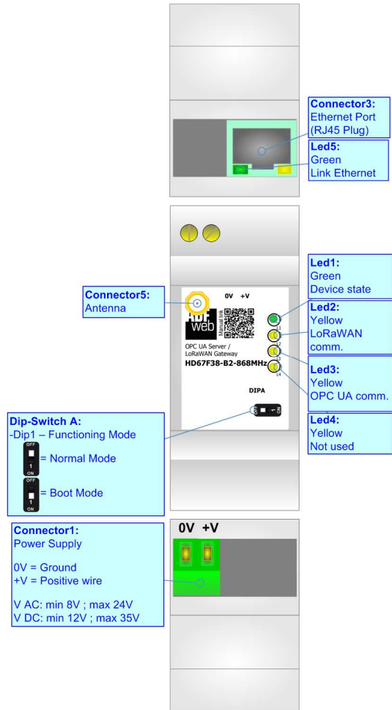
Figure 1: Connection scheme for HD67F38-B2-xxxMHz
