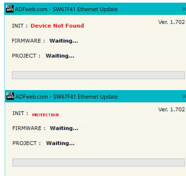
Figure 7: "Error" window
