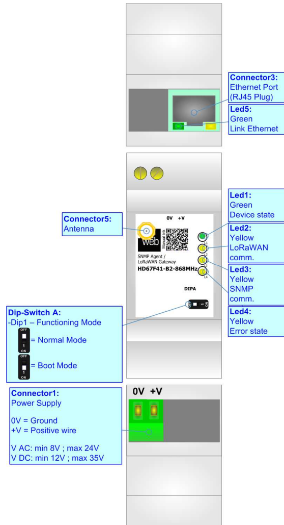
Figure 1: Connection scheme for HD67F41-B2-xxxMHz
